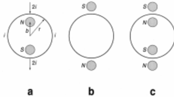
Fig. 2. Schematics (a) of Wesley's version of the Marinov motor (top view of ring rotor and solenoids, with current direction reversed, brush contact locations indicated), (b) of a modification in which solenoids, with reversed polarities, are situated outside the ring, (c) superposition of cases (a) and (b).
